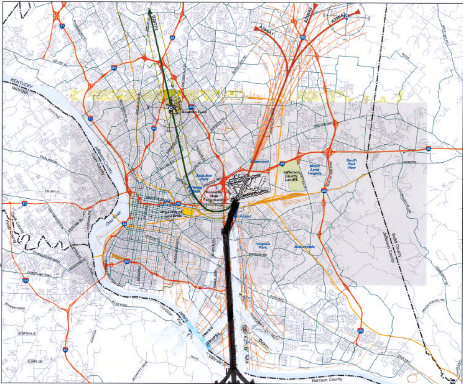
Figure H ARRIVAL AND DEPARTURE FLIGHT TRACKS—RUNWAY 29 FAR Part 150 Noise Compatibility Study Louisville International Airport
